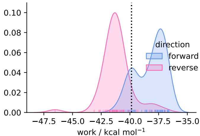
solvent ( N = 59 )
