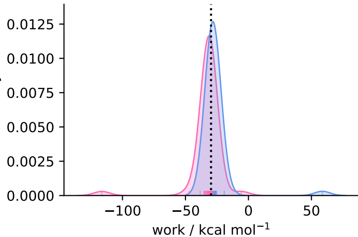
complex ( N = 44 )
