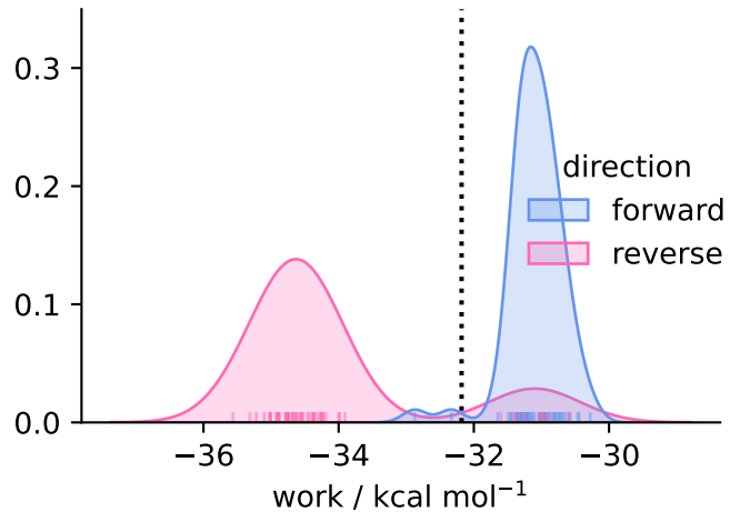
solvent ( N = 60 )
