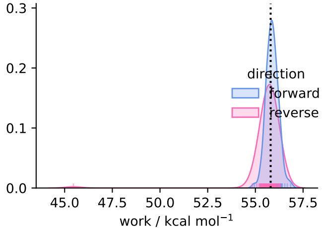
solvent ( N = 99 )
