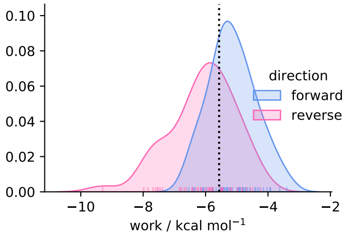
solvent ( N = 50 )
