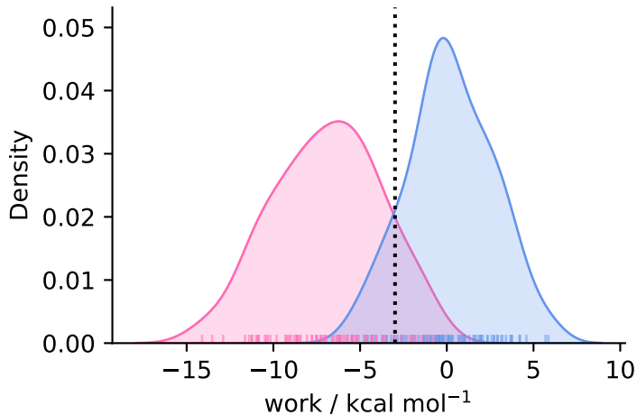
complex ( N = 80 )
