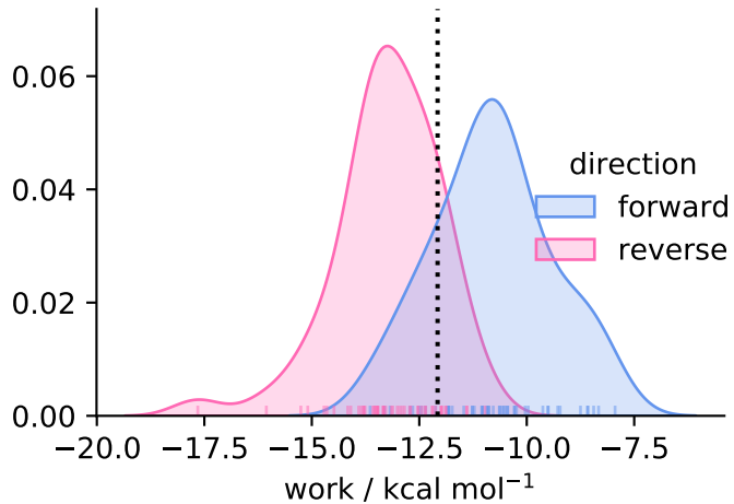
solvent ( N = 49 )
