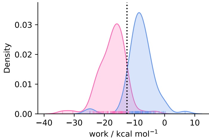
complex ( N = 77 )
