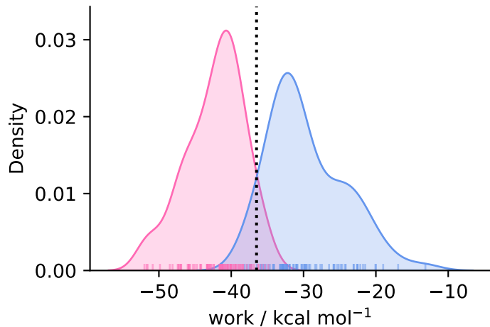
complex ( N = 79 )
