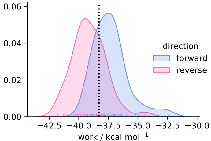
solvent ( N = 50 )
