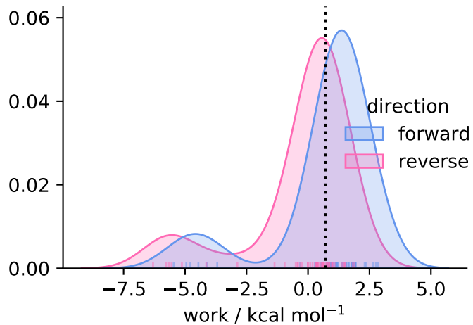
solvent ( N = 49 )
